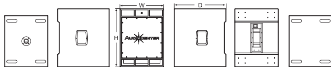
Dimension(W×H×D):520×700×618mm
