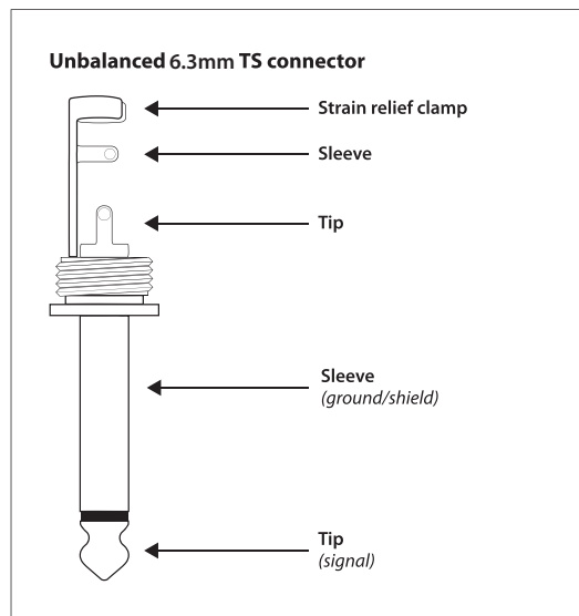
Fig. 4.3: TS connector
