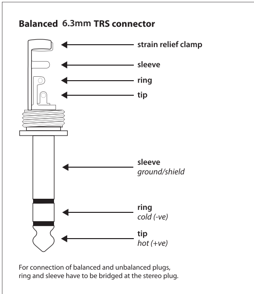
Fig. 4.4: TRS connector
